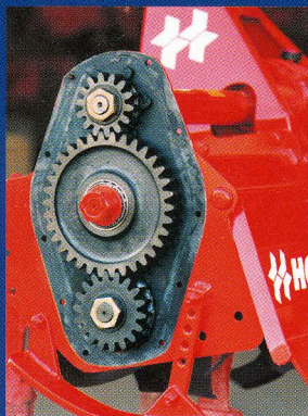
Detail of side drive gears.
