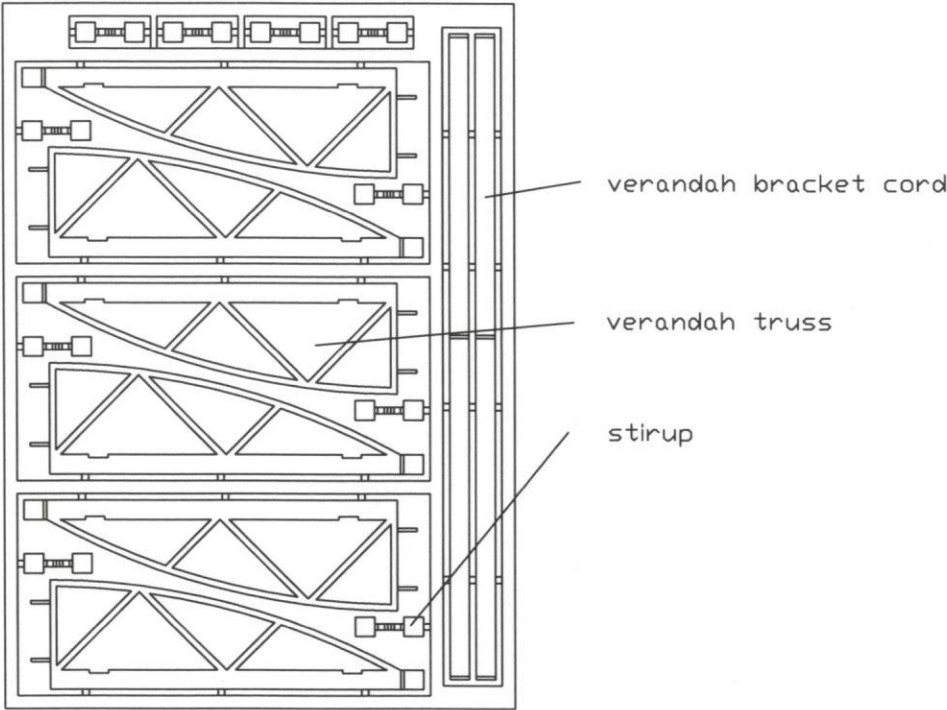
280 mm Verandah Frame
