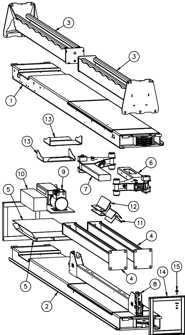
Fig 2 – Package Components
