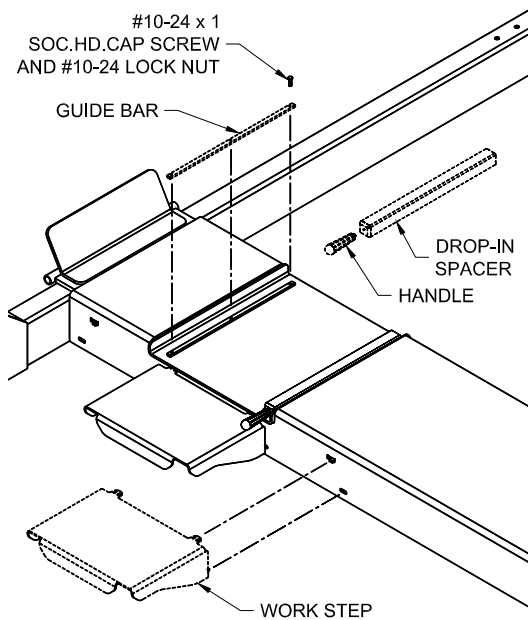
Fig 19 – Alignment Turn Plate Installation
