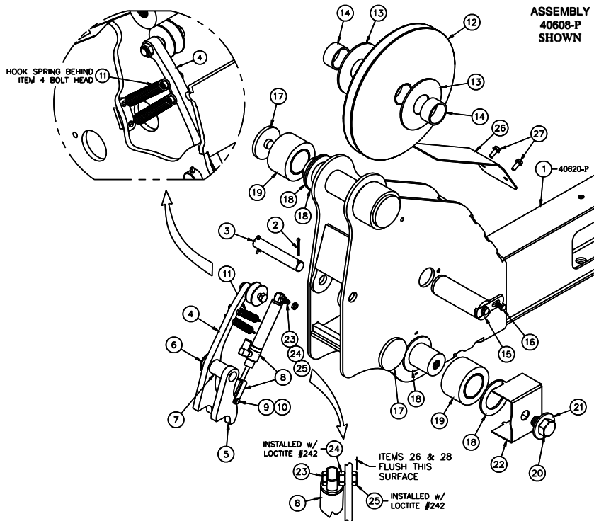
Fig E. Front Cross Beam
