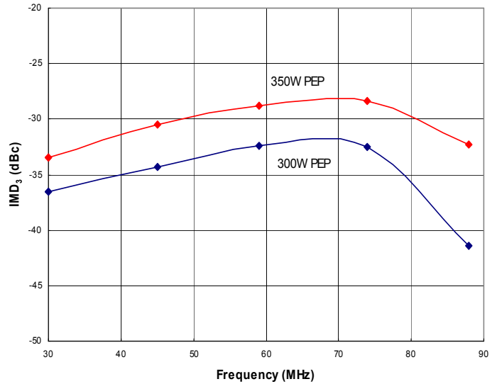
Figure 2: RFP30-88-350XR Typical IMD 3 @ 350W and 300W PEP, Δf=100kHz and Δf=10kHz.
