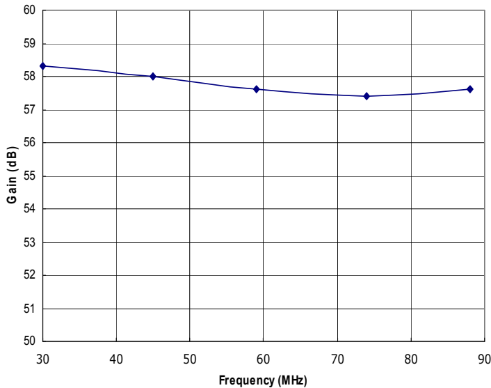
Figure 1: RFP30-88-350XR Typical Gain @ P out =350W.
