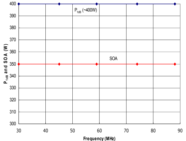
Figure 4: RFP30-88-350XR Typical P 1dB and Safe Operating Area (SOA). The SOA assumes a 50 ohm load and adequate cooling of output transformers. Do not exceed the SOA shown above without first contacting RFMPT to discuss your application.
