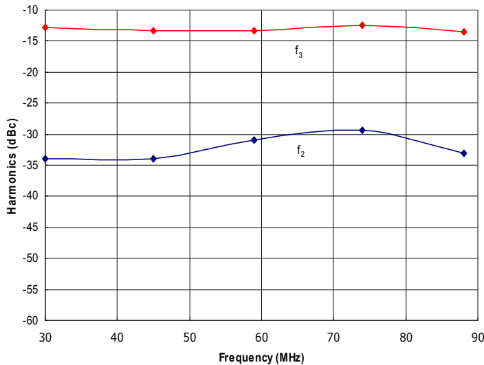
Figure 3: RFP30-88-350XR Typical f 2 and f 3 @ P out =350W.
