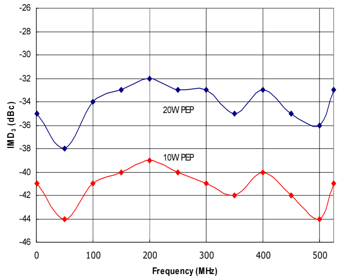
Figure 2: RFMS1-525-20 Typical IMD_3 , \Delta f=10kHz , @ P_{out} = 20W and 10W PEP.
