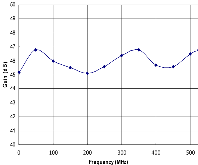
Figure 1: RFMS1-525-20 Typical Gain @ P_{out} = 20W .
