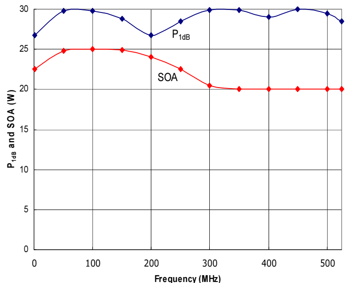
Figure 4: RFMS1-525-20 Typical P_{1dB} and Safe Operating Area (SOA). The amplifier is capable of delivering more power than it is safe to generate. Do not exceed the SOA without first contacting RFMPT to discuss your application.
