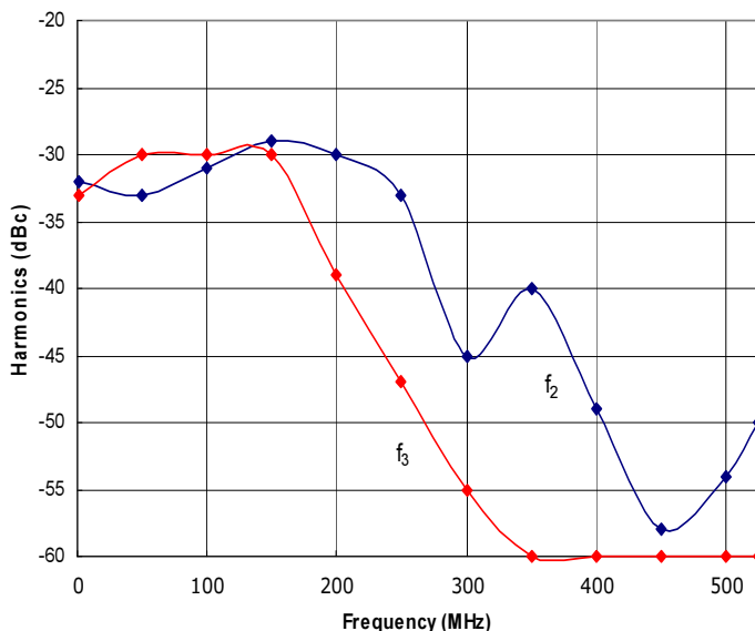
Figure 3: RFMS1-525-20 Typical f_2 and f_3 @ P_{out} = 20W .
