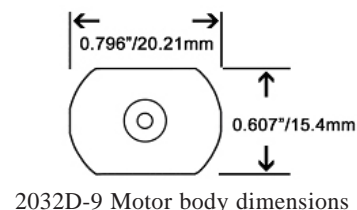
2032D-9 Motor body dimensions
