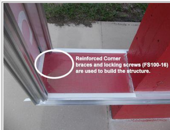
TS44 Structure Here a monument realized with mesh vinyl
