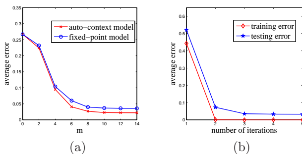
Figure 1. (a): comparison of the testing errors on the OCR dataset by varying m ; (b): the training and testing errors on the OCR dataset as \mathcal{T} varies.
