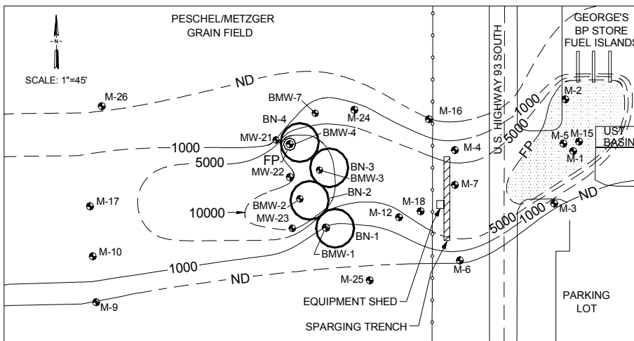
FIGURE 2. Site map before BioNet treatment.
