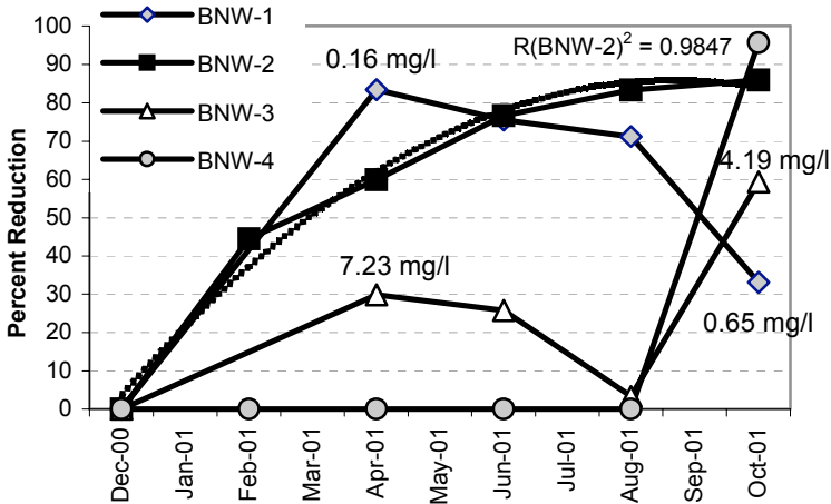
FIGURE 5. Percent reduction of MTBE in BioNets.
