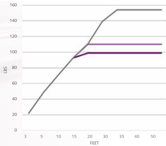
SHUTTLE HD (M) AND SHUTTLE Z-WAVE
