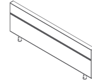
Desk Mounted Screen ZF-F40-W08 800×T40×H350(fit W1200 Desk) ZF-F40-W10 1000×T40×H350(fit W1400 Desk) ZF-F40-W11 1100×T40×H350(fit W1500 Desk) ZF-F40-W12 1200×T40×H350(fit W1600 Desk)
