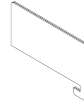
Side Screen--Acoustic Panel ZF-PET-D060 550×T18×H370(fit D600 Desk) ZF-PET-D070 650×T18×H370(fit D700 Desk) ZF-PET-D080 750×T18×H370(fit D800 Desk)
