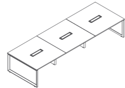
Conference Table M10-T04-1212 3600×1200×H750 M10-T04-1214 3600×1400×H750
