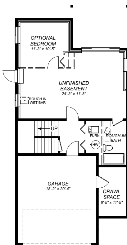
LOWER FLOOR PLAN 782 sq ft
