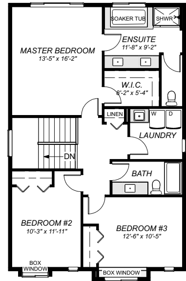
UPPER FLOOR PLAN 1055 sq ft
