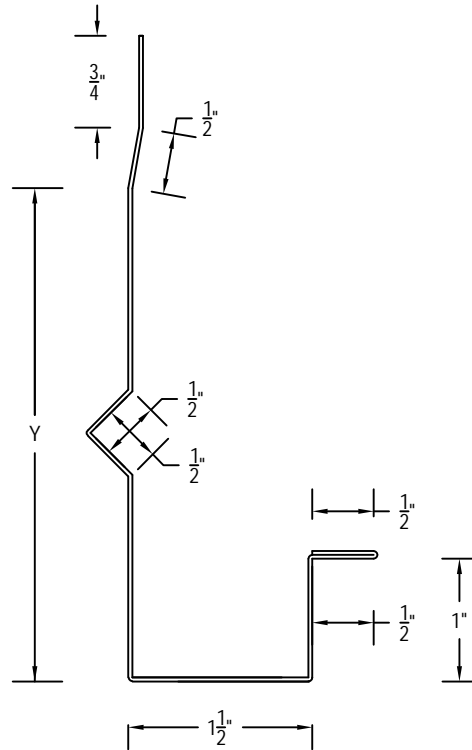
J-FASCIA WITH STIFFENER & RETURN _____ LINEAR FEET (120" PCS)
