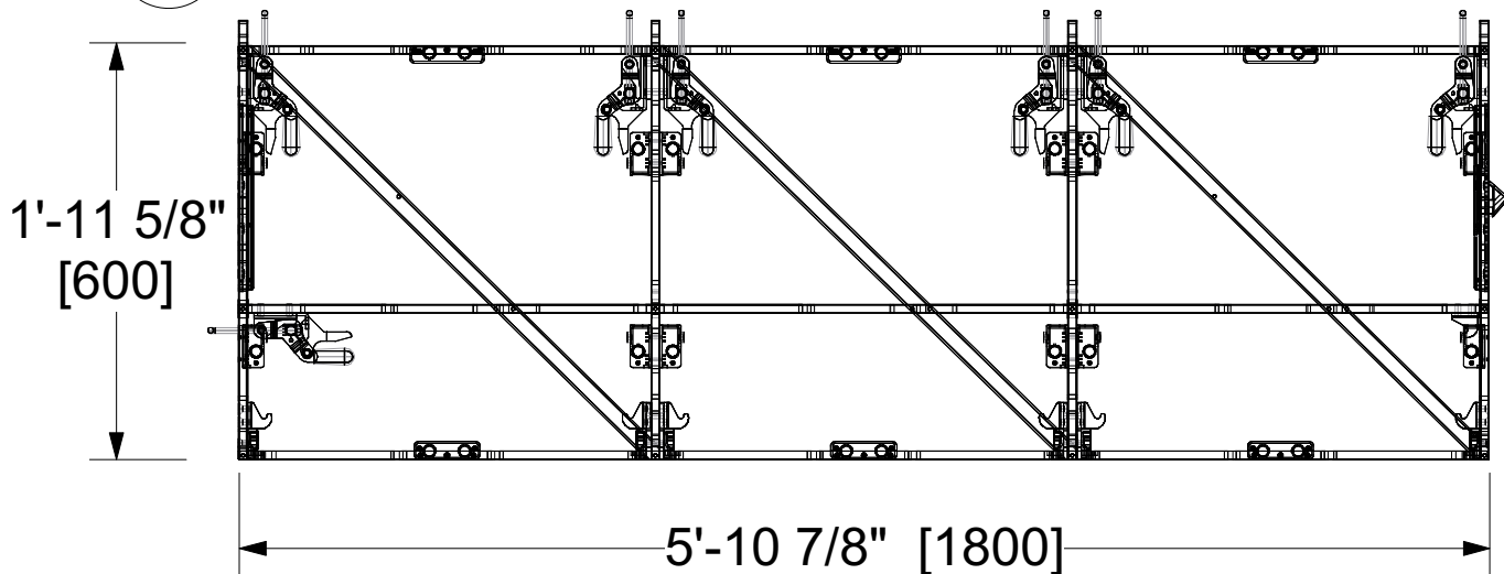
1 Front View 1" = 1'0"
