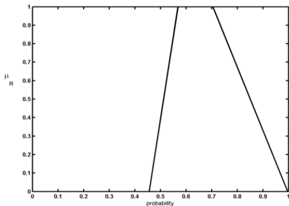
Fig.8: Fuzzy reliability of Mltipath omega network of size (16 x 16)
