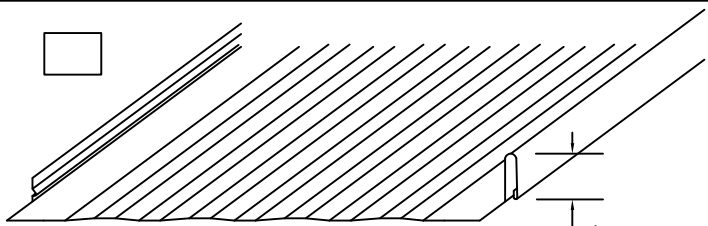
1-1/2" SNAP SEAM PANEL WITH STRIATIONS 11-1/2", 15", (16-7/8") AND 19-1/2" WIDE PANEL PRE-NOTCHED
