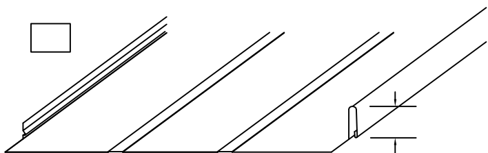
1-1/2" SNAP SEAM PANEL WITH 2 LOW FLAT BEADS 11-1/2", 15", (16-7/8") AND 19-1/2" WIDE PANEL PRE-NOTCHED
