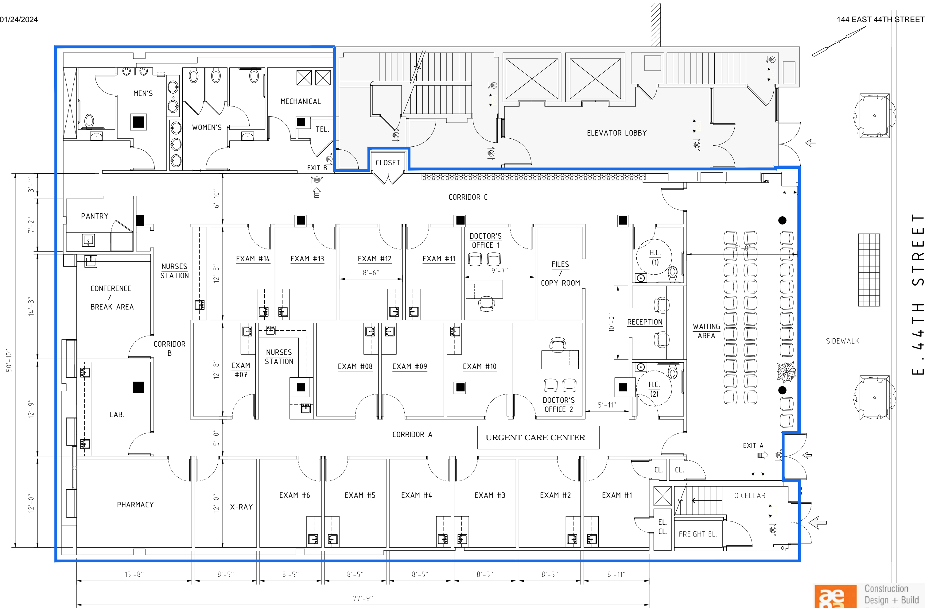
FIRST FLOOR PLAN - A
