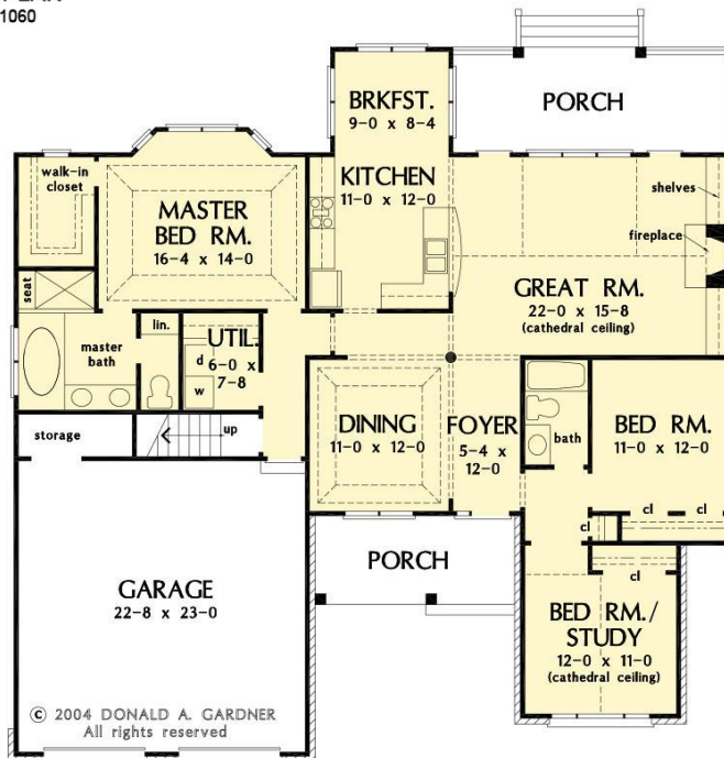
FLOOR PLAN PLAN NO. 1060
