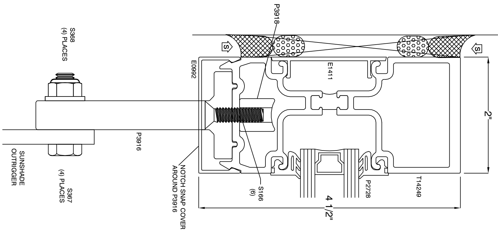
M1 MAXBLOCK ANCHOR @ JAMB -
