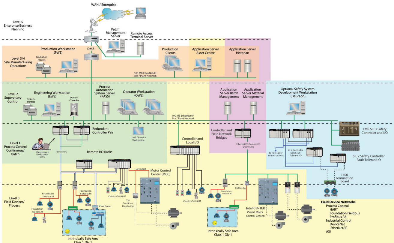
Diagram 1: Multidiscipline Control System Architecture
