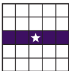
Row Example
