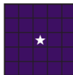
Blackout Example
