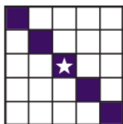
Diagonal Example
