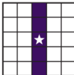
Column Example
