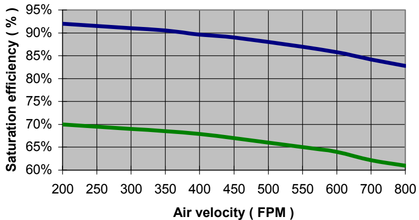
Efficiency: AluCool 4" and 8" Pads
