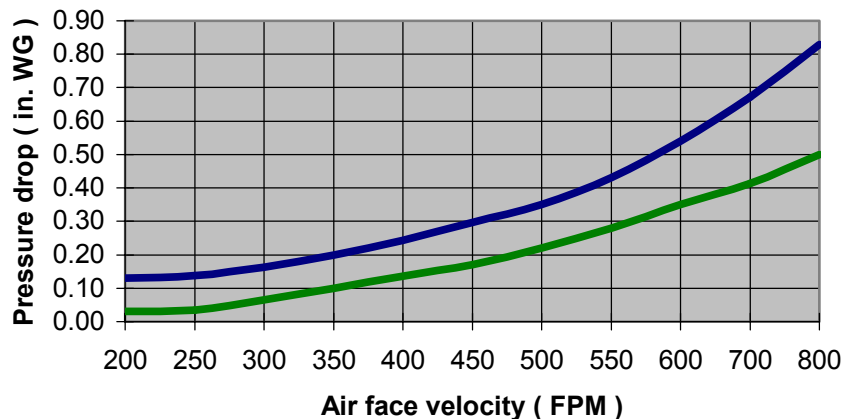
Pressure Drop MII AluCool 4" and 8" Pads
