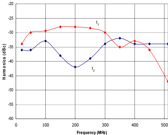
Figure 3: RFM20-512-50-HSD Typical f_2 and f_3 @ P_{out}=50W .
