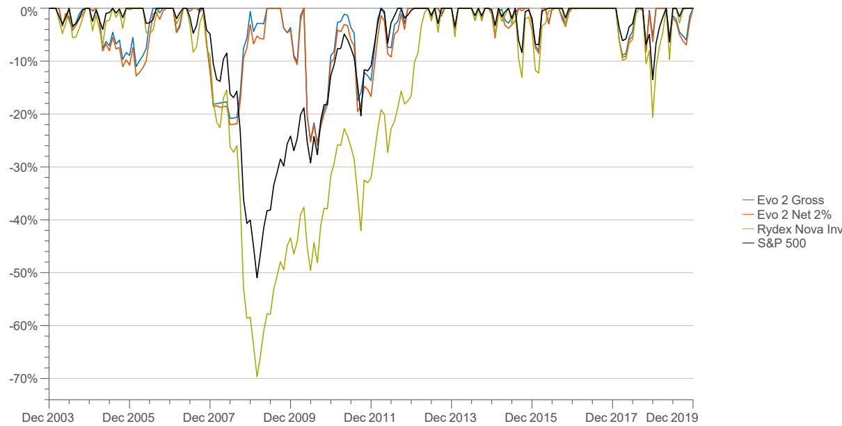
Drawdown January 2004 - December 2019
