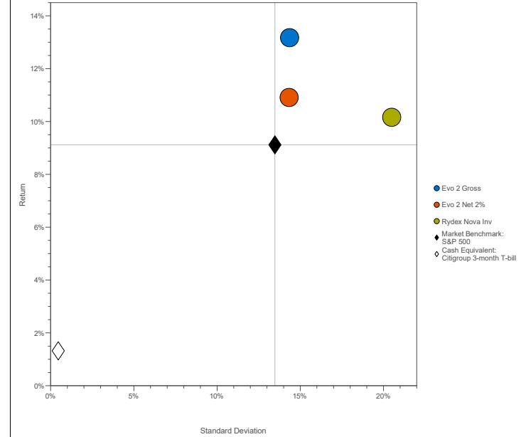
Risk / Return January 2004 - December 2019 (Single Computation)
