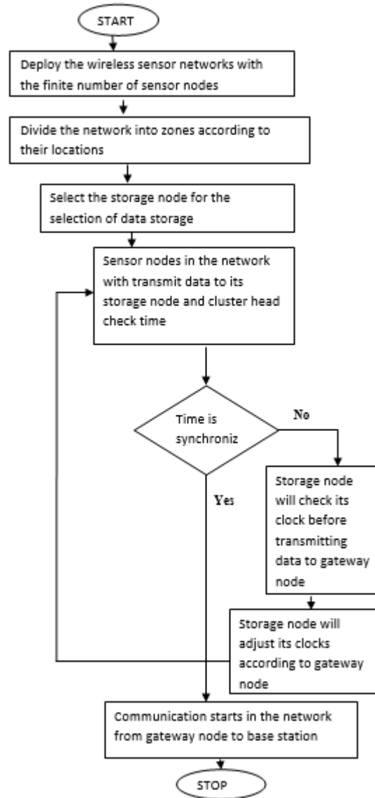
Fig 1: Proposed Methodology
