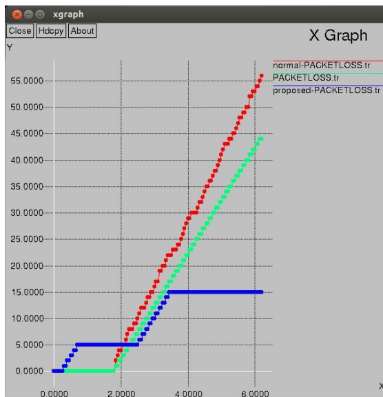
Fig 2: Packetloss Graph
