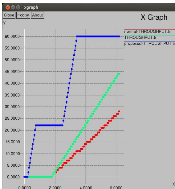
Fig 3: Throughput Comparison
