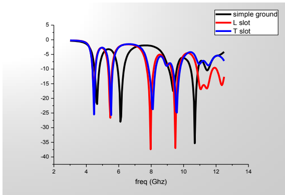
Fig. 2 Results with different slots in ground
