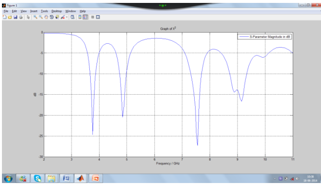
Fig. 7 Analysis results through PSO
