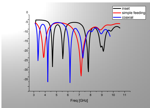
Fig. 3 Results with different feedings
