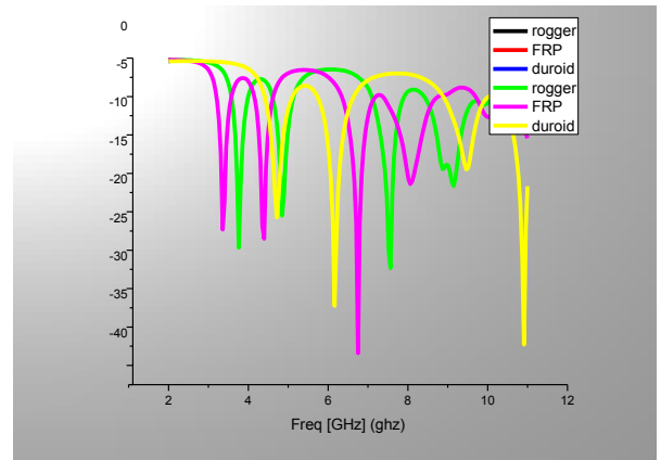
Fig. 4 Results with different substrate material
