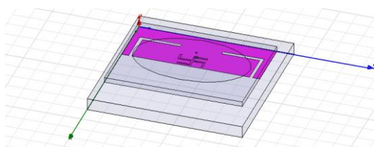
Fig. 1 L-slot design
