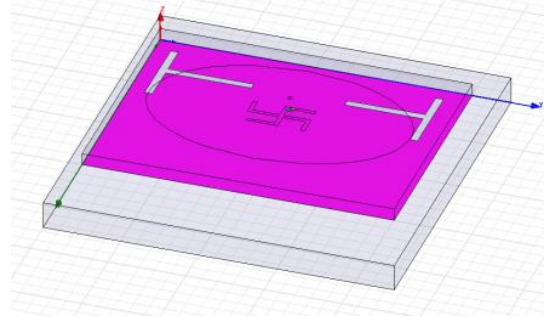
Fig. 2 T-slot design
