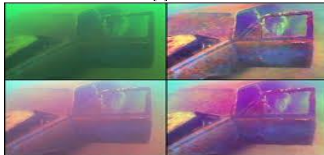
Fig.7: Histogram equalization
