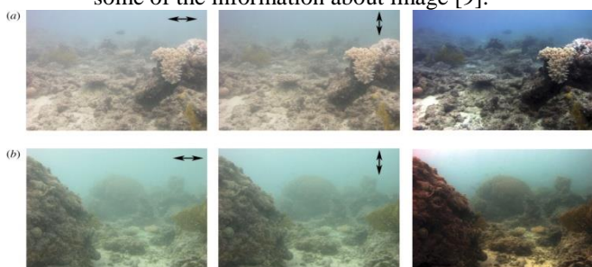
Fig.1: Visibility Restoration
