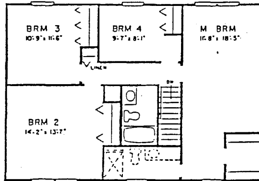
SECOND FLOOR PLAN (Four Bedroom Model)
