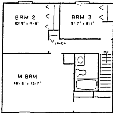
SECOND FLOOR PLAN (Three Bedroom Model)
