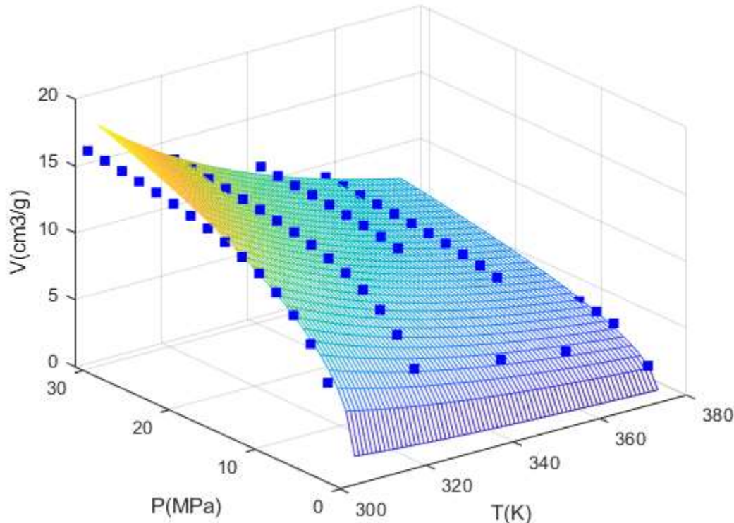
Figure 1: The measured adsorption values and TPAE surface of fat coal
