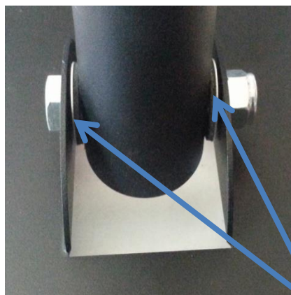
Washer Isolators
