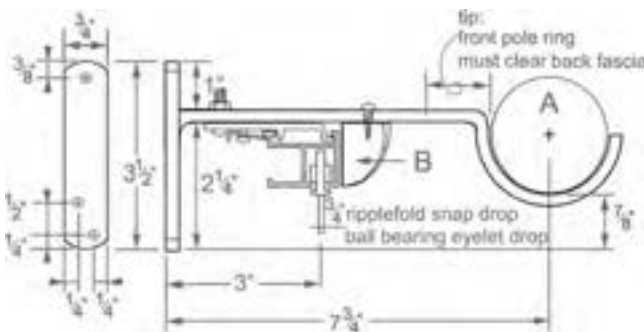
BBOVBKS Ball Bearing Over Bracket
