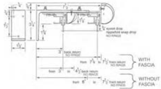
BB51 Adjustable 6"- 7" Double Bracket
