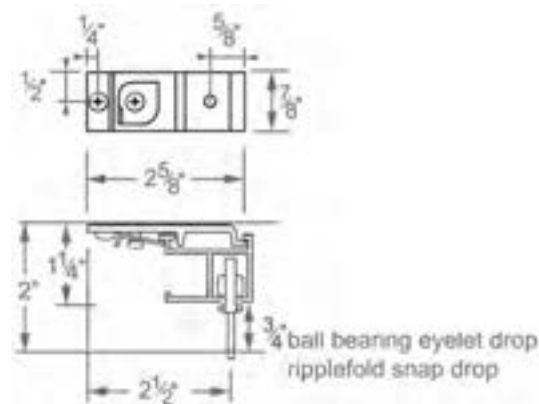
BBCM Single Ceiling Mount Bracket
