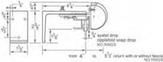
BB50 Adjustable 4"- 5 1/4" Single Bracket
