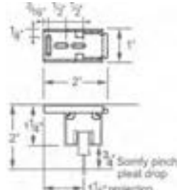
Somfy Ceiling Mount Bracket Available in White only
