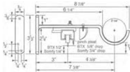
Motorized Over-Bracket Portfolio and Quick Ship Wood and Resin finishes only. Sold separately. Use with Single Motorized Track.
