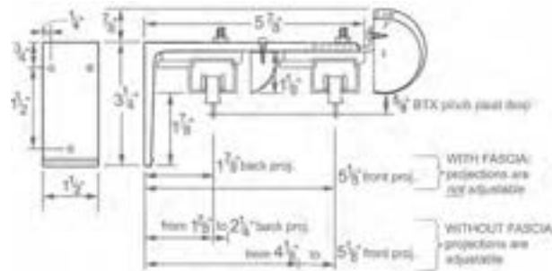
Somfy Double Motorized Bracket Available in Gold, Bronze or White
