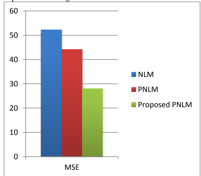
Fig.3: MSE Comparisons
