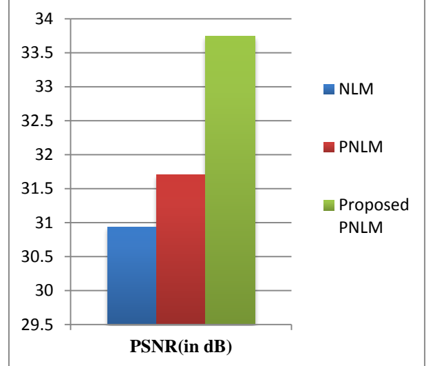
Fig.2: PSNR Comparison
