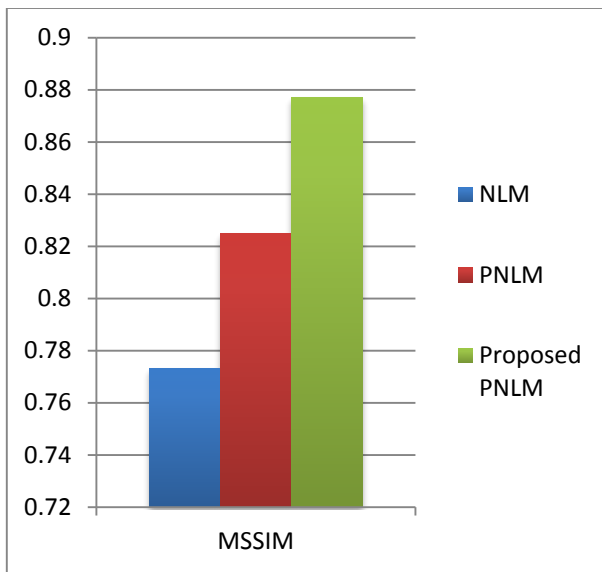
Fig.4: MSSIM Comparison
