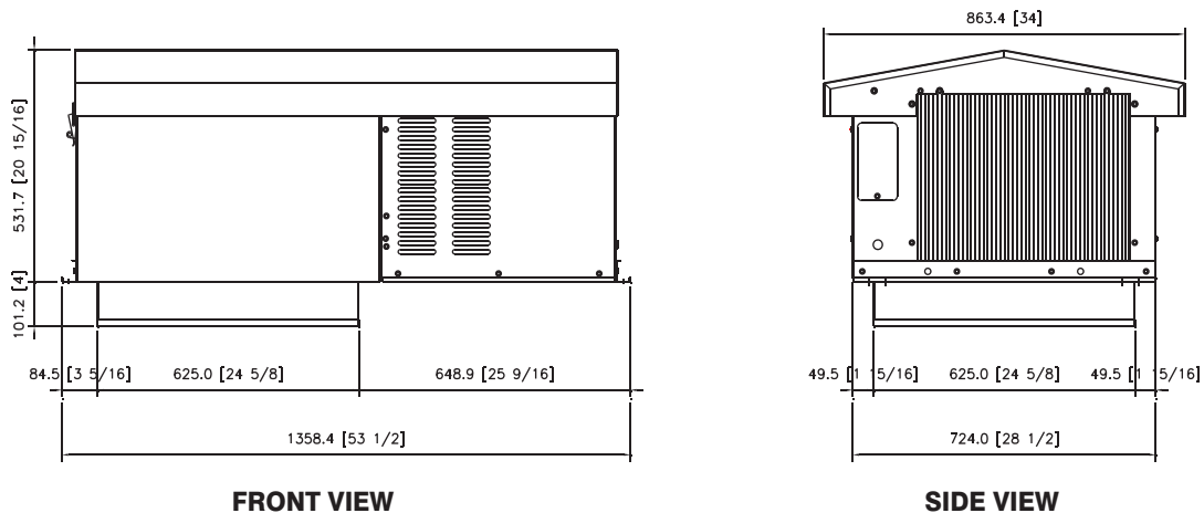
Figure B. INDOOR UNIT – Medium Cabinet (Opening Size : 25 inch x 25 inch)
