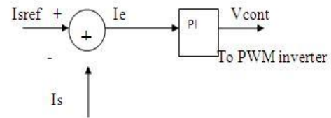
Fig3: Inner current loop
