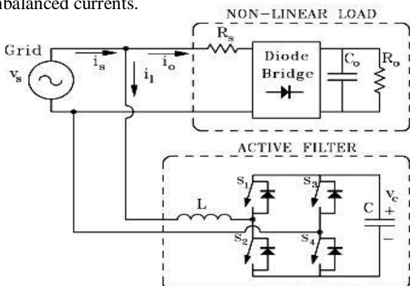
Fig2: Shunt APF with non-linear load and the full-bridge converter
