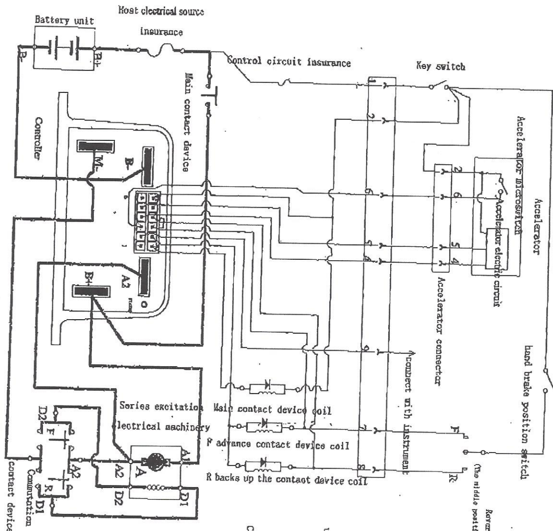
Controller unit wiring diagram
