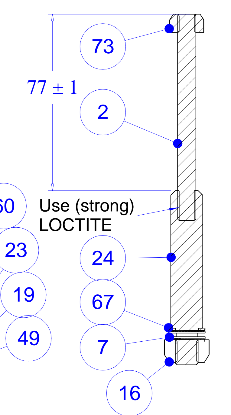
CROSS SECTION DEPTH CONTROL SHAFT
