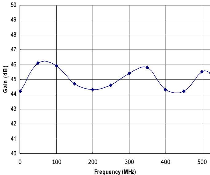
Figure 1: RFM1-525-20 Typical Gain @ P_{out} = 20W .
