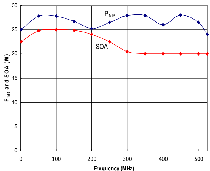
Figure 4: RFM1-525-20 Typical P_{1dB} and Safe Operating Area (SOA). The amplifier is capable of delivering more power than it is safe to generate. Do not exceed the SOA without first contacting RFMPT to discuss your application.
