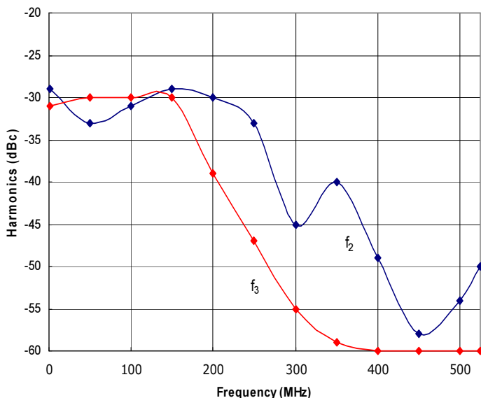
Figure 3: RFM1-525-20 Typical f_2 and f_3 @ P_{out} = 20W .
