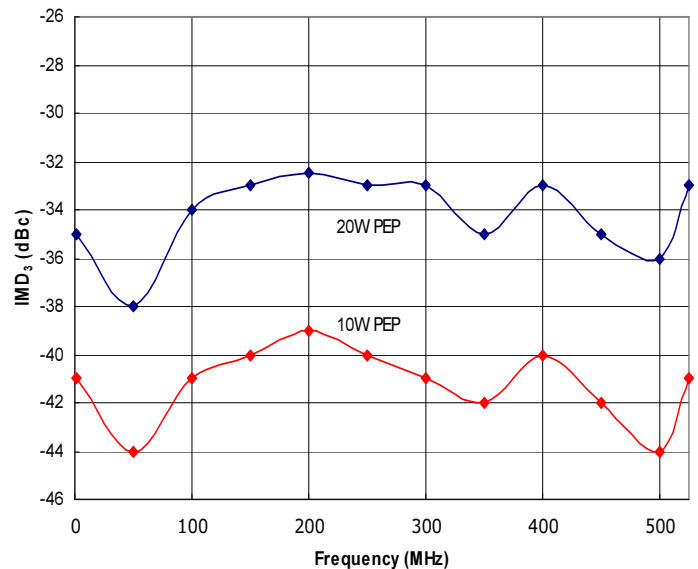
Figure 2: RFM1-525-20 Typical IMD_3 , \Delta f=10kHz , @ P_{out} = 20W and 10W PEP.
