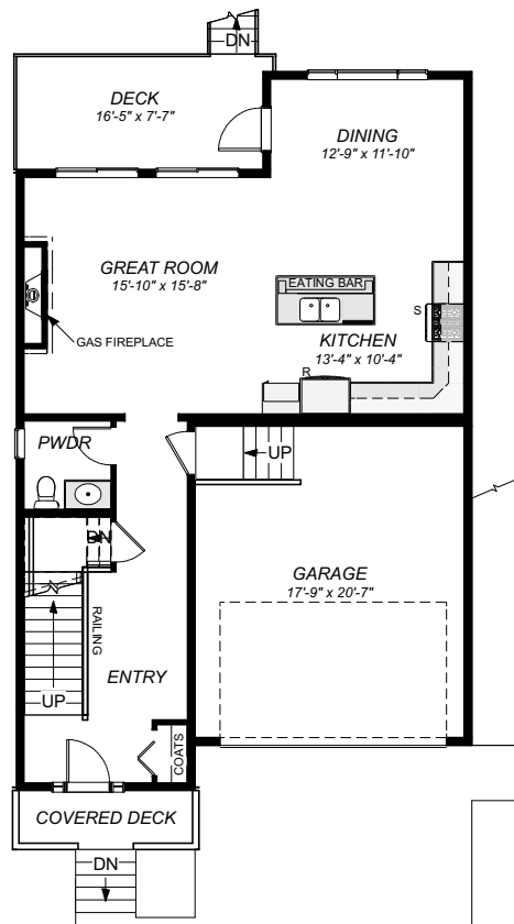
MAIN FLOOR PLAN 889 sq ft
