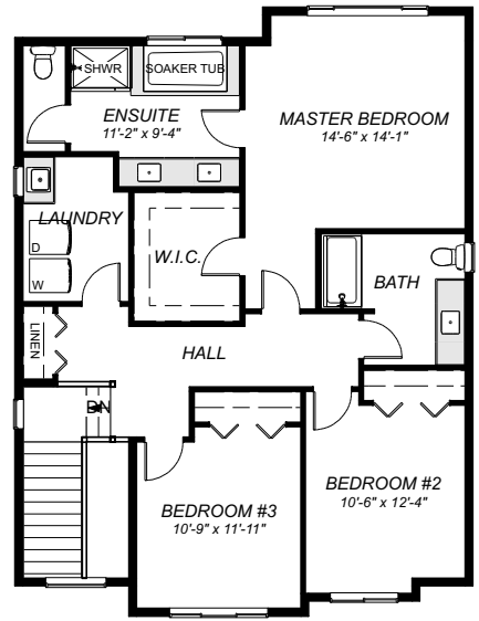
UPPER FLOOR PLAN 1150 sq ft
