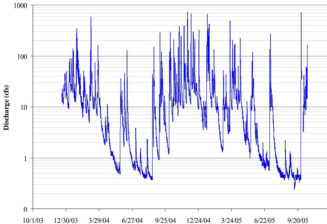
Figure 4.85. Provisional Coal Creek discharge data (source: MFM, unpublished hydrologic data).
