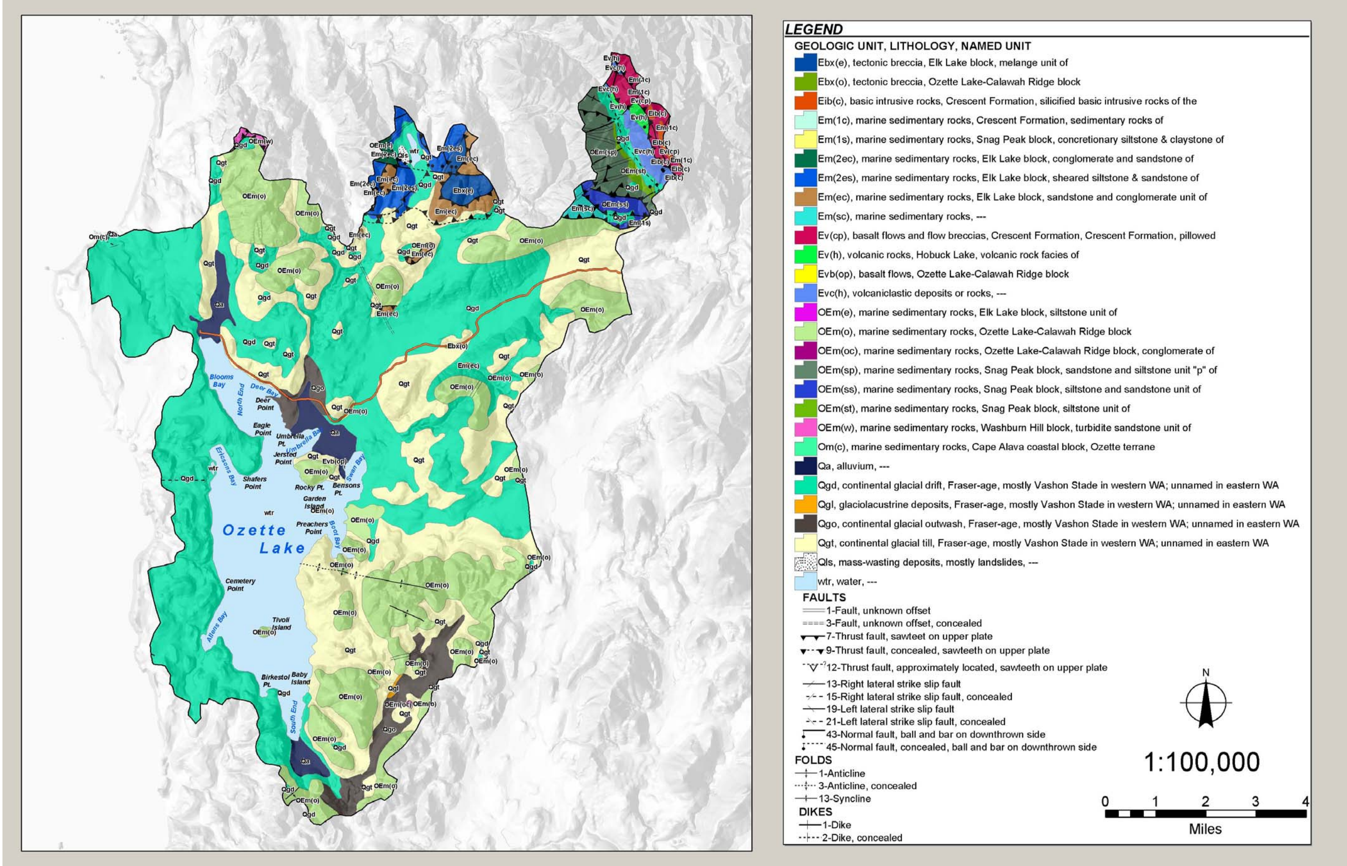
Figure 1.3. Ozette watershed geology (source: Schasse2003)
