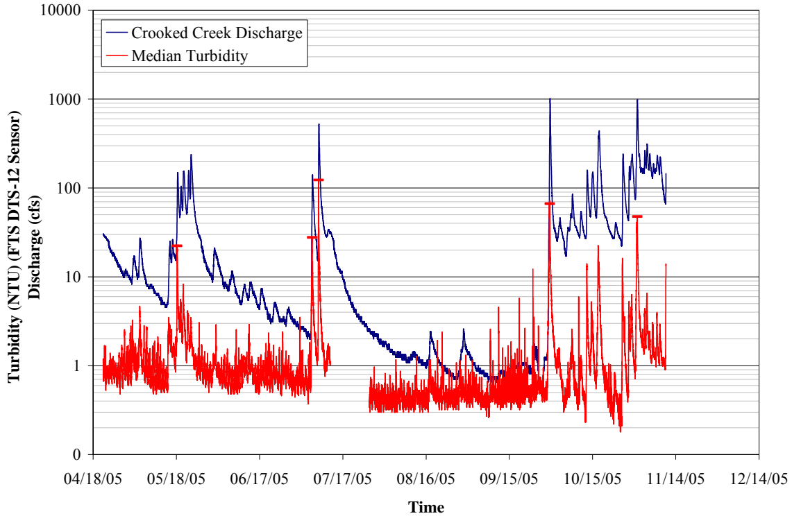
Figure 4.89. Provisional Siwash Creek continuous turbidity data contrasted with Crooked Creek stream discharge data (source: MFM, unpublished data).
