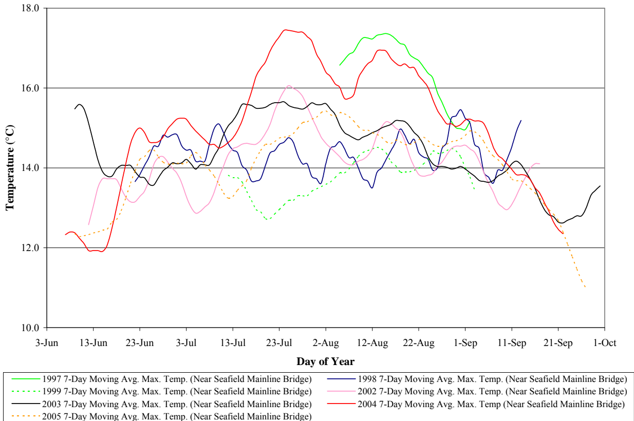
Figure 4.79. Coal Creek 7-day moving average maximum stream temperature near Seafield Mainline Bridge (MFM, Green Crow, and QNR, unpublished stream temperature data).
