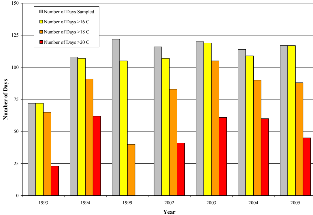
Figure 4.31. Number of days sampled and the number of days stream temperature exceeded 16, 18, and 20 °C in the Ozette River from 1993 through 2005 (source: MFM unpublished stream temperature data; Meyer and Brenkman 2001).
