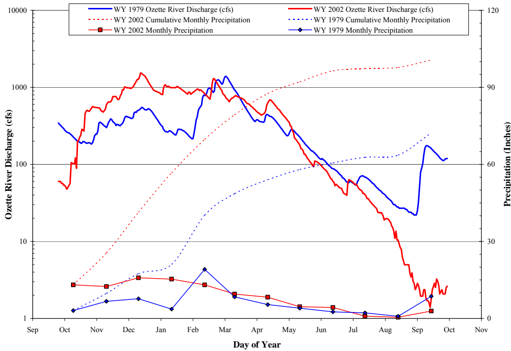
Figure 5.10. Comparison of Ozette River WY 1979 and WY 2002 streamflow discharge and monthly and cumulative water year precipitation at Quillayute Airport (source: USGS and MFM, published and unpublished streamflow data; NOAA-NCDC 2005).
