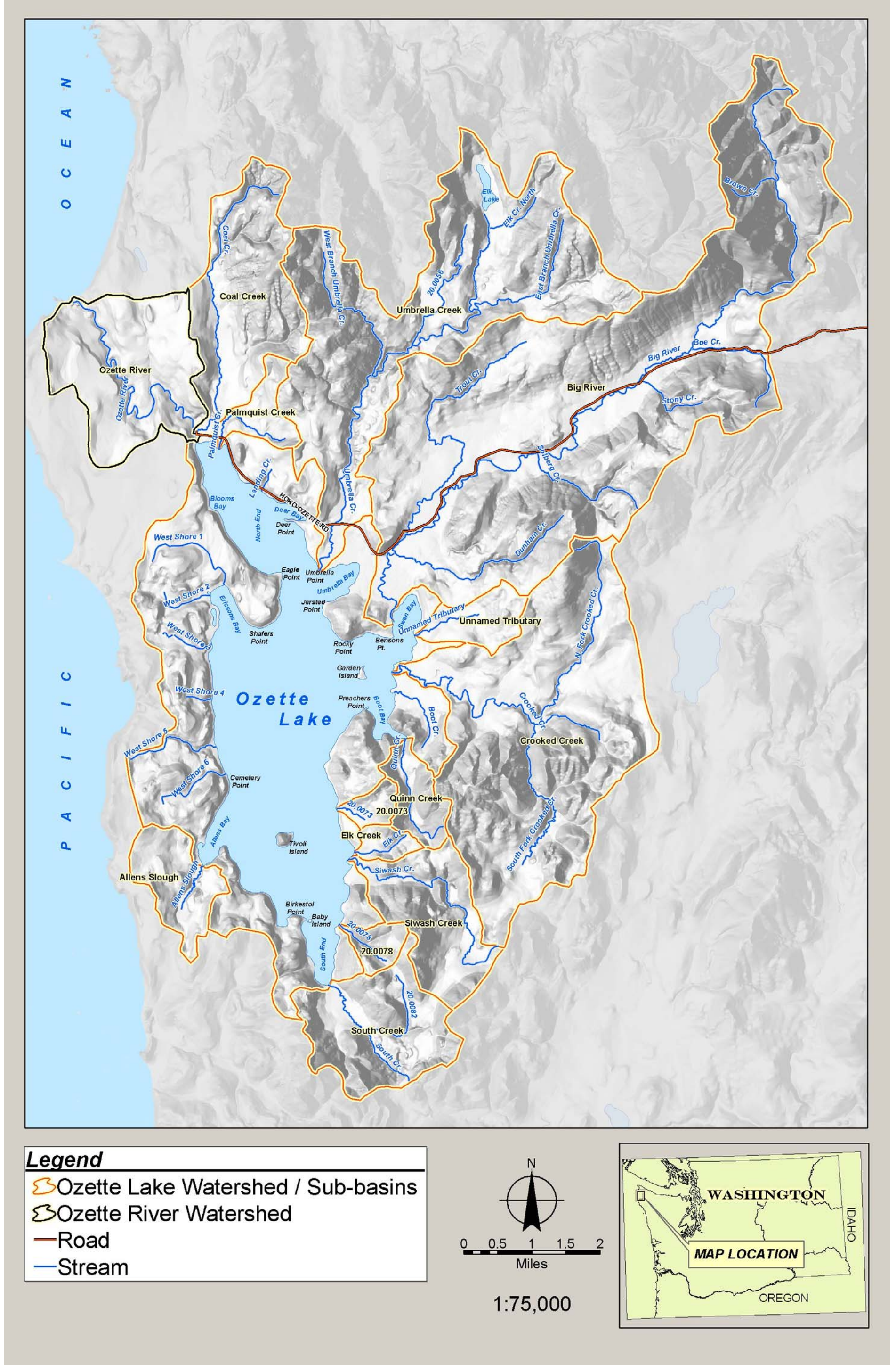
Figure 1.1. Lake Ozette watershed overview map (source: original hydrography from DNR Hydro GIS layer).
