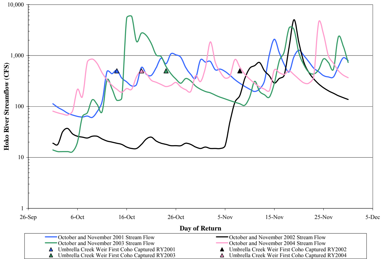
Figure 2.5. Relationship between streamflow 8 and the first coho salmon captured in the Umbrella Creek weir for return years 2001 through 2004 (source: hydrologic data from USGS gage 12043300; biological data from MFM, unpublished weir records).
