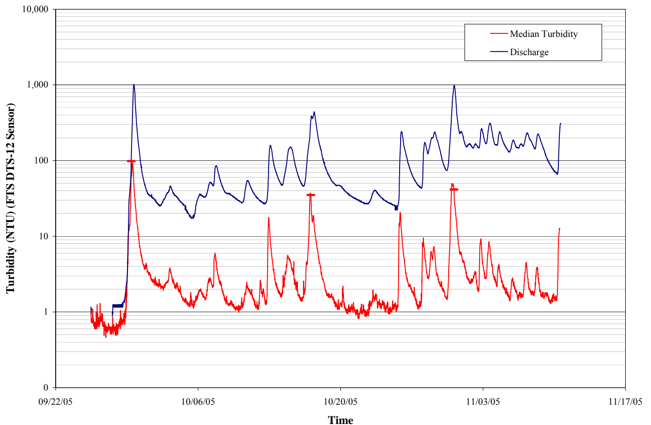
Figure 4.72. Preliminary results from continuous turbidity readings and provisional stream discharge data for Crooked River (source: MFM, unpublished data).
