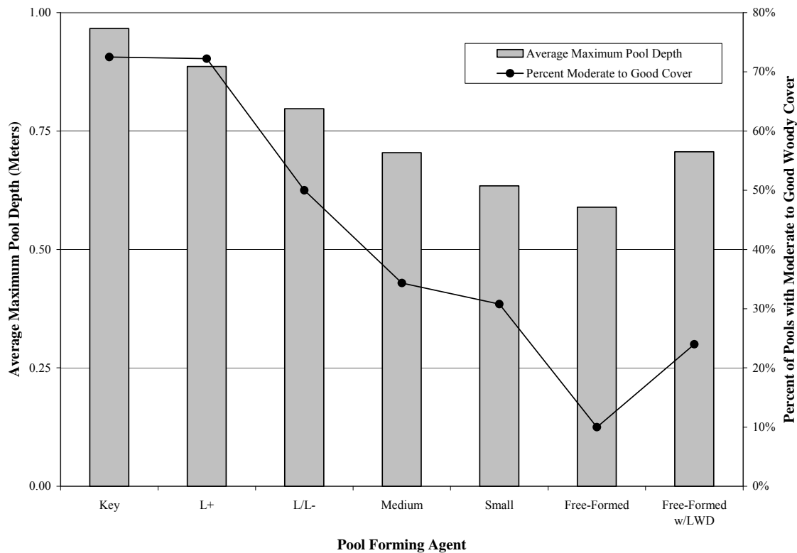
Figure 4.76. Relationship between primary pool forming agent and pool depth and percent pool cover for Coal Creek (source: Haggerty and Ritchie 2004). Note: L+ = LWD > 50 cm diameter and > 5 m length; L/L- = LWD > 50 cm diameter < 5 m length; medium = LWD 50-20 cm diameter; small = LWD 10-20 cm diameter; moderate woody cover = 6-20% cover; and good woody cover = > 20% woody cover.
