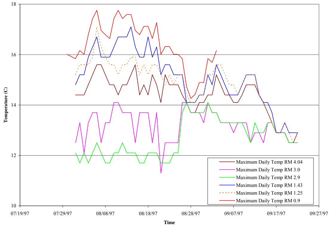
Figure 4.77. Coal Creek maximum daily stream temperature at six sites during the summer of 1997 (source: MFM and Green Crow, unpublished data).
