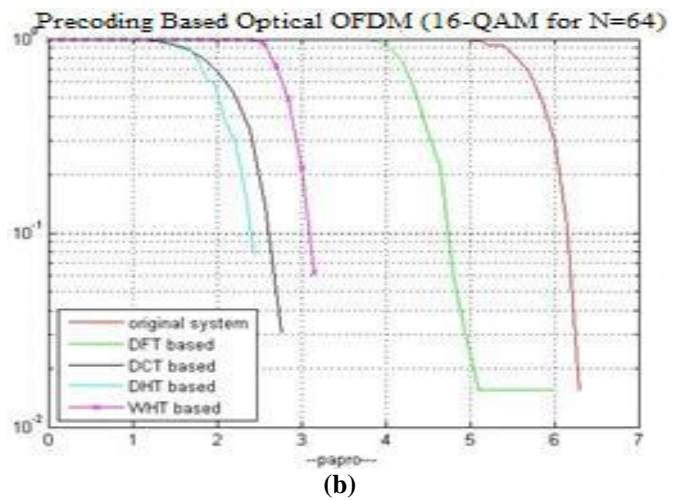
Fig.2 (a), (b) PAPR analysis of proposed and existing schemes
