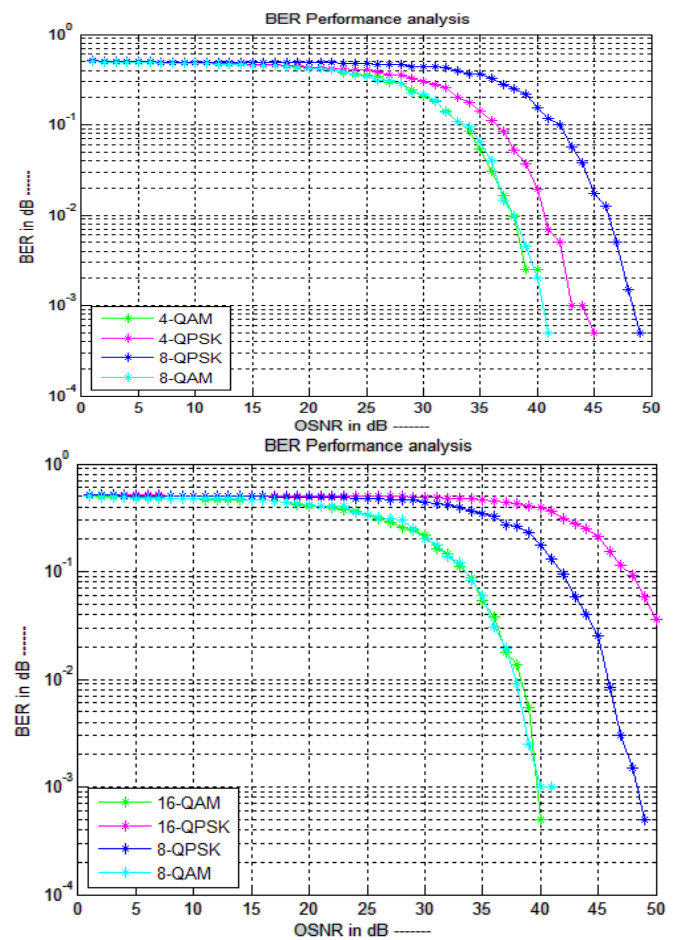
Fig.3: BER performance of different modulation schemes
