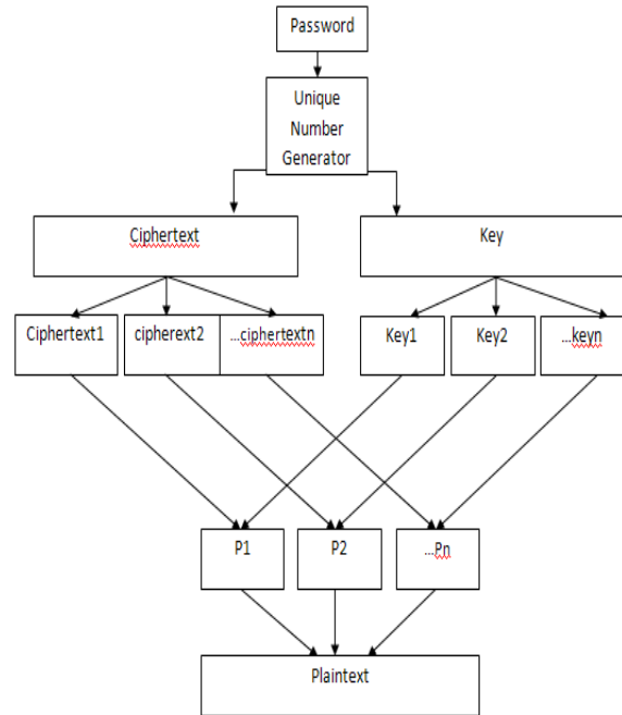
Fig.4: Split-file -key pair algorithm –Decryption
