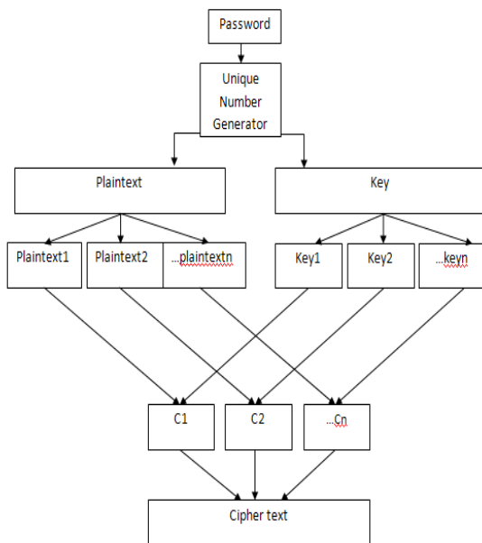
Fig.3: Encryption
