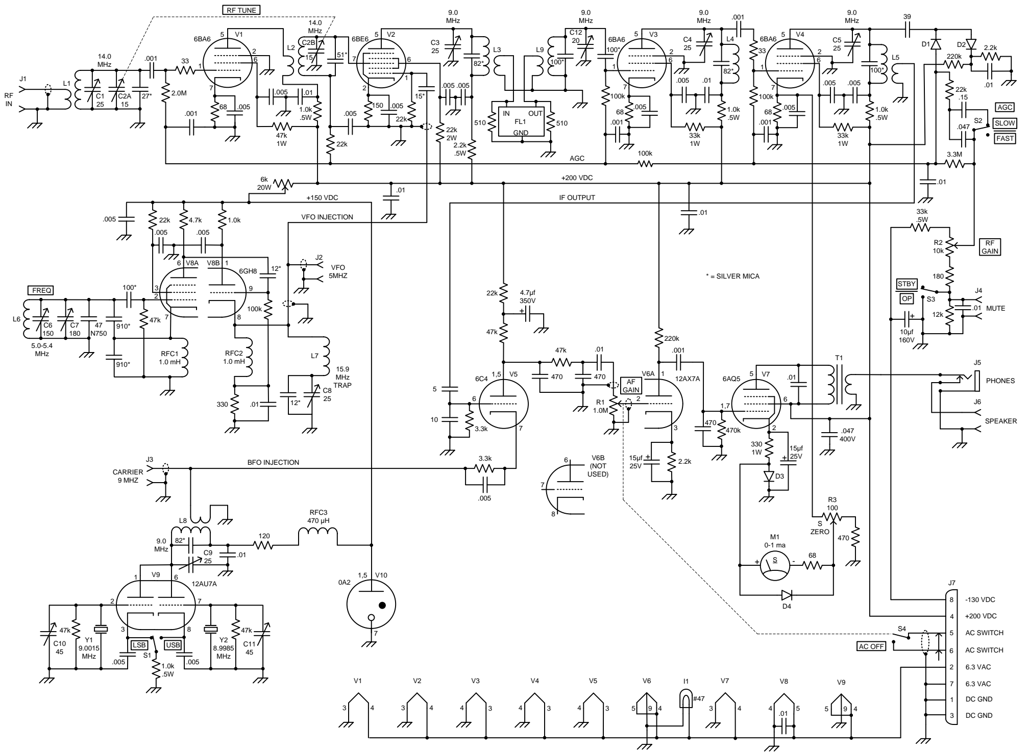
RECEIVER SCHEMATIC
