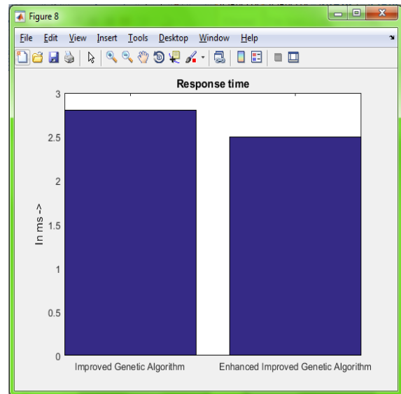
Fig 1: Comparison graph of Response Time
