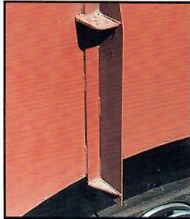
Side fins inside the tub help move material away from the edge of the tub and into the path of the cylinder.
