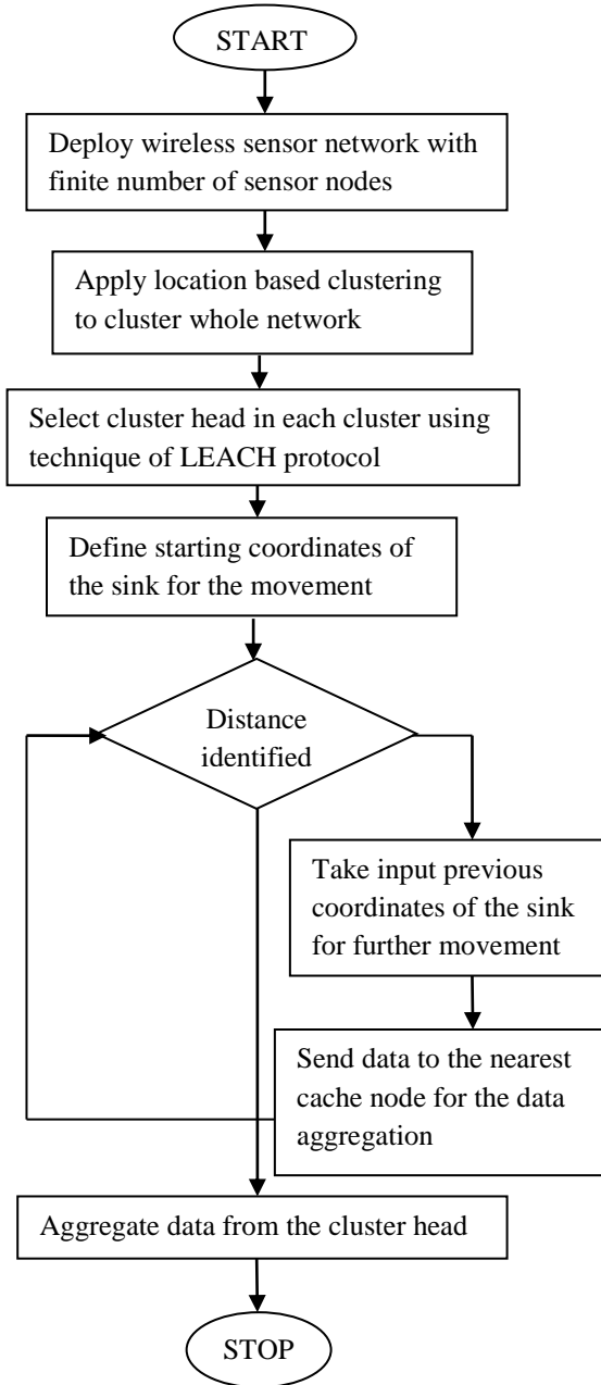
Fig.1: Proposed Flowchart
