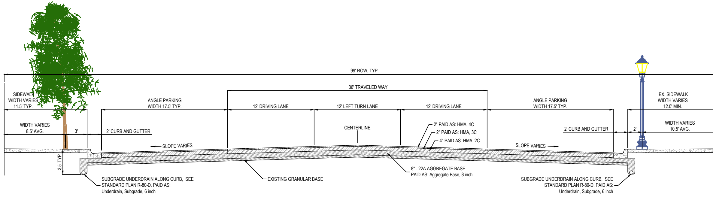
2 DRYDEN RD - PROPOSED TYP ROAD CROSS SECTION SCALE: NONE
