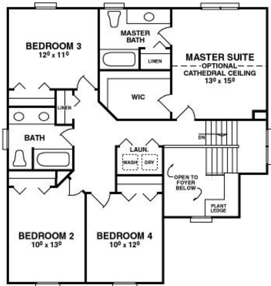
SECOND FLOOR PLAN W/OPTIONAL 4TH BEDROOM
