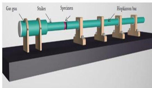
Fig.28: Hopkinson Pressure Bar Set-Up [10].
