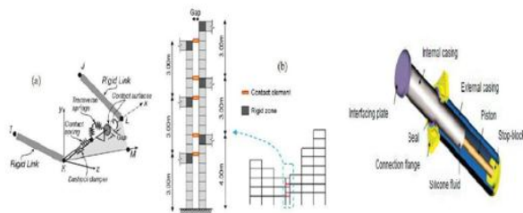
Fig.29: Ruaumoko Contact Element [11]. Fig.30: Piston type contact element [12].
