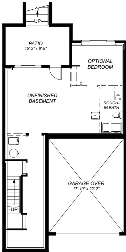
LOWER FLOOR PLAN 873 sq ft
