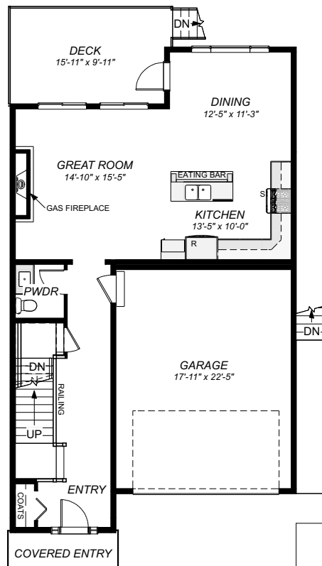
MAIN FLOOR PLAN 870 sq ft
