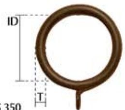
RING 350 ID = Internal Diameter T = Thickness
